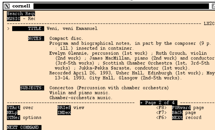
Figure 2. Terminal emulator after several queries to Cornell University Library
